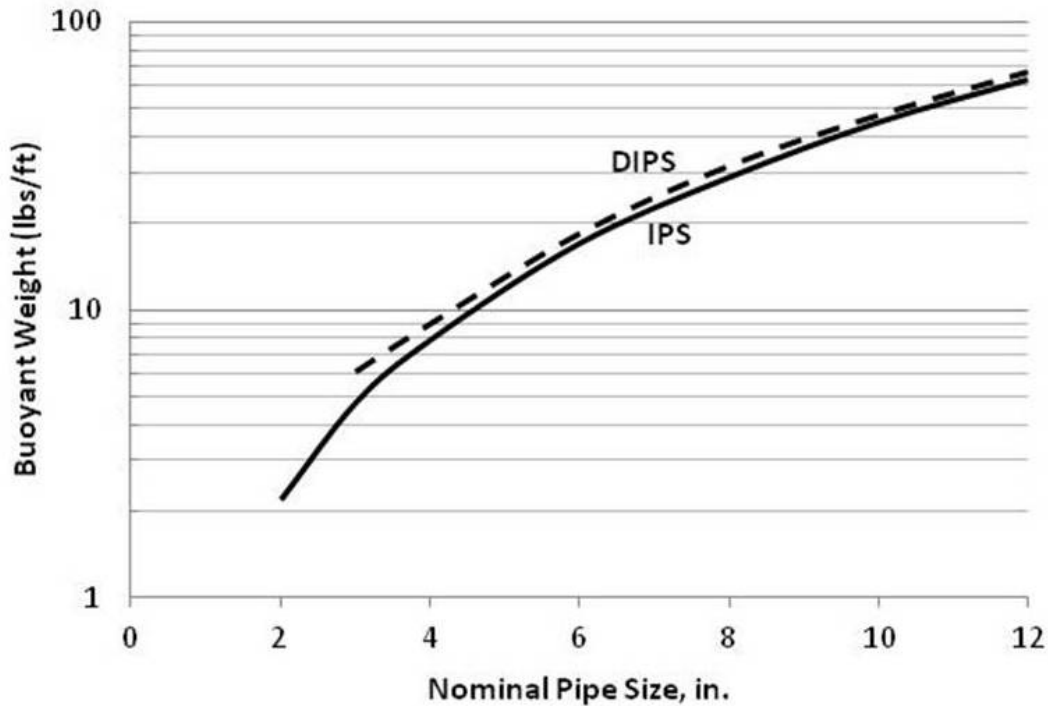
Figure 7 Buoyant Weight of HDPE Pipe (Source: Outside Plant Consulting Services, Inc.)
