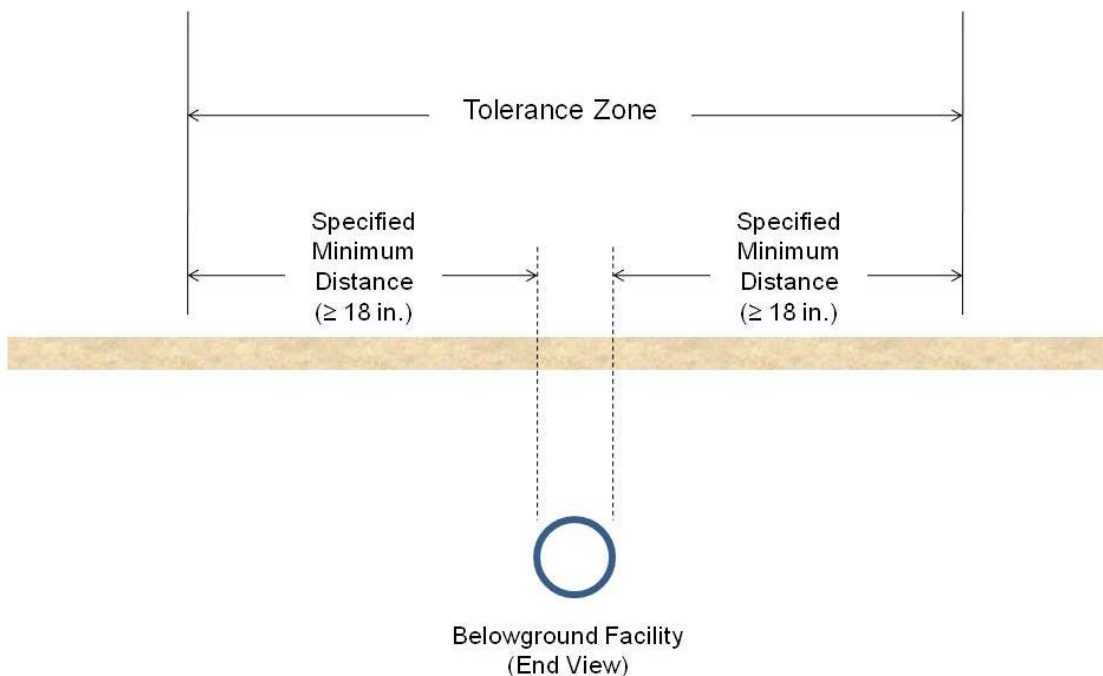
Figure 5 Tolerance Zone
