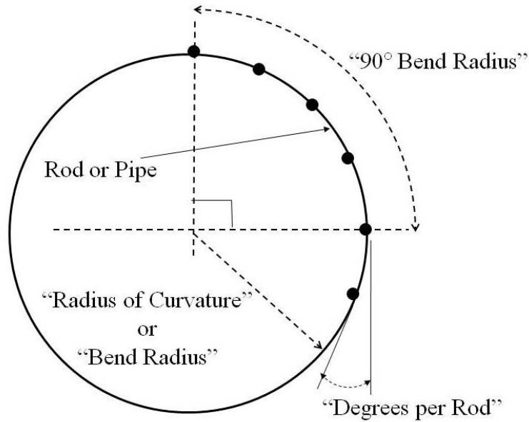
Figure 3 Rod or Pipe Curvature Terminology (Source: Outside Plant Consulting Services, Inc.)
