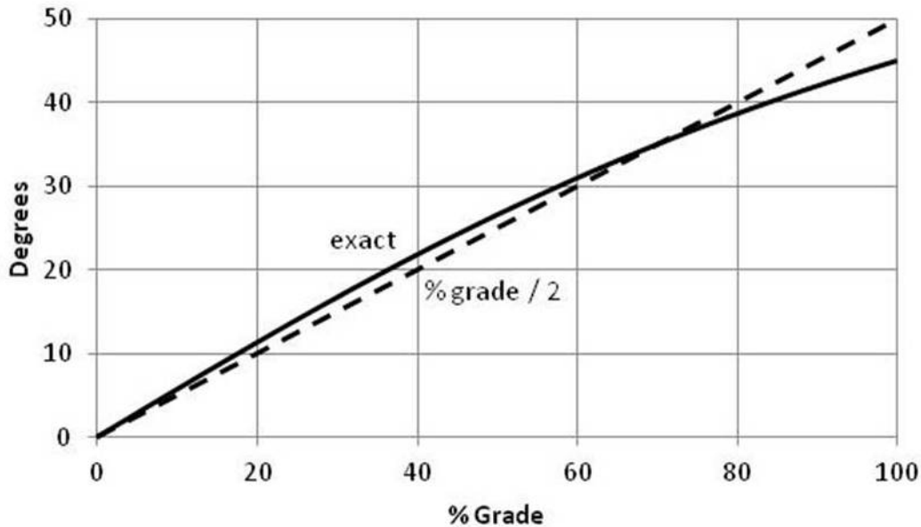
Figure 12 Degrees vs. Percent Grade
