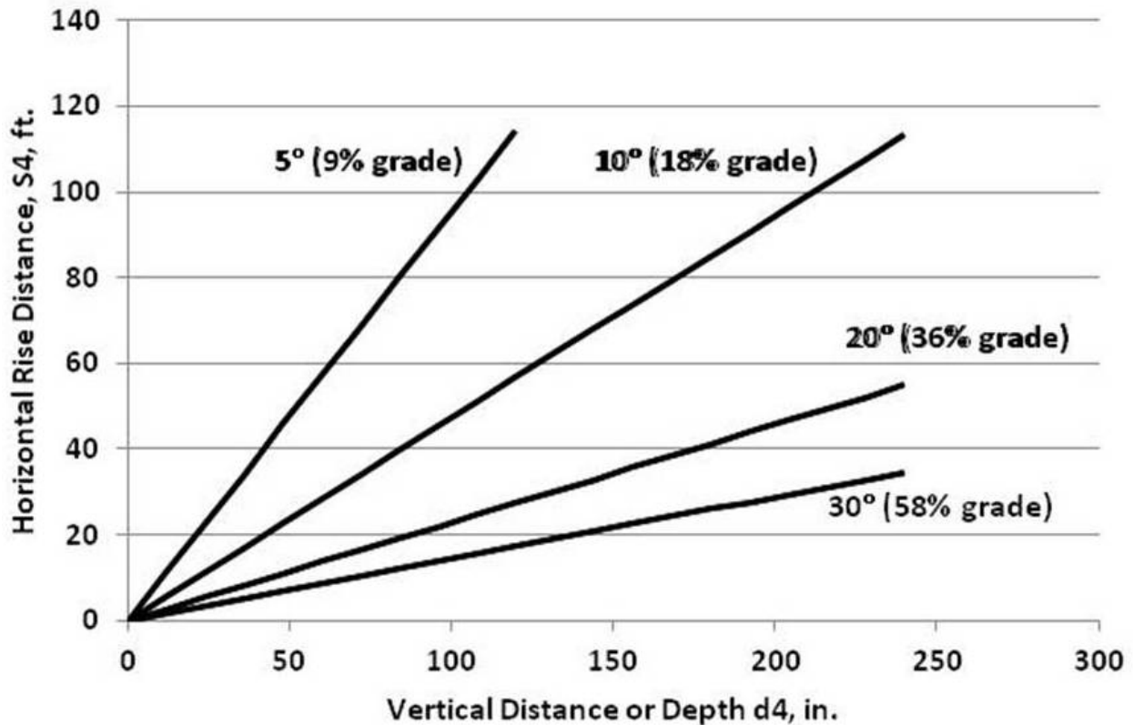
Figure 20 Horizontal Distance to Rise Vertical Distance or to Surface
