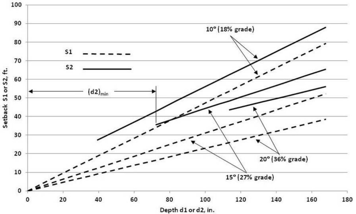
Figure 14 Drill Rig Setback Distance Drill Rods: 10 ft Long, 100 ft Radius of Curvature (Source: Outside Plant Consulting Services, Inc.)
