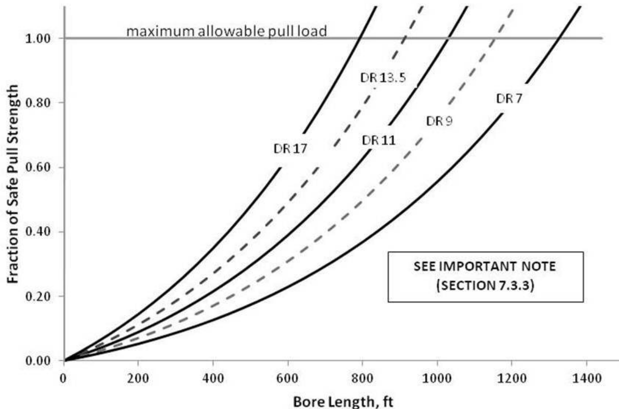
Figure 9 Predicted Mini-HDD Pull Load vs. Safe Pull Tension, HDPE (PE4710) Pipe Nominally Straight Path, 2-inch Drill Rods (Source: Outside Plant Consulting Services, Inc.)
