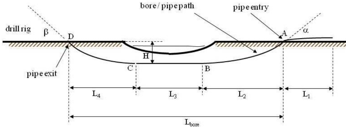
Figure C.1 Nominal Maxi-HDD Route (River Crossing) (Source: Outside Plant Consulting Services, Inc.)
