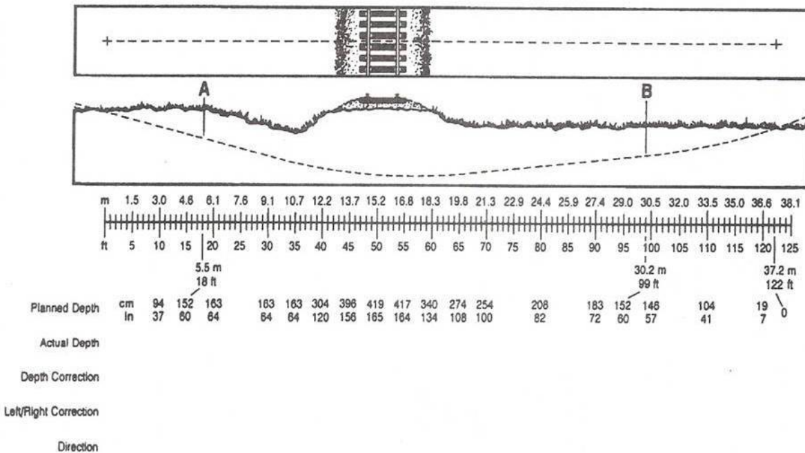
Figure 22 Initial Bore Plan (Source: Ditch Witch®)
