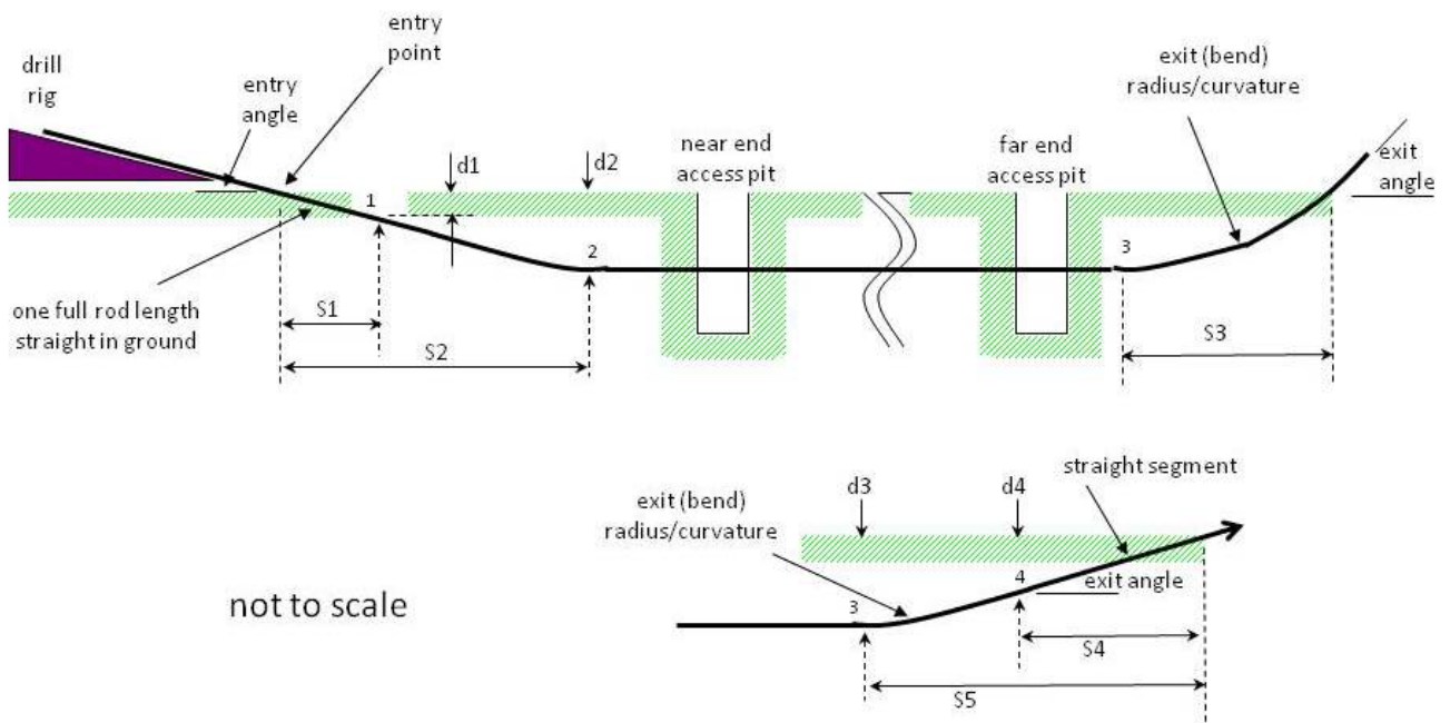
Figure 11 Drill Rig Setup and Related Distances (Source: Outside Plant Consulting Services, Inc.)
