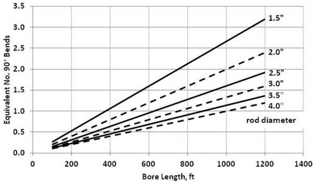
Figure 8 Unplanned Curvature, n_2 (Source: Outside Plant Consulting Services, Inc.)
