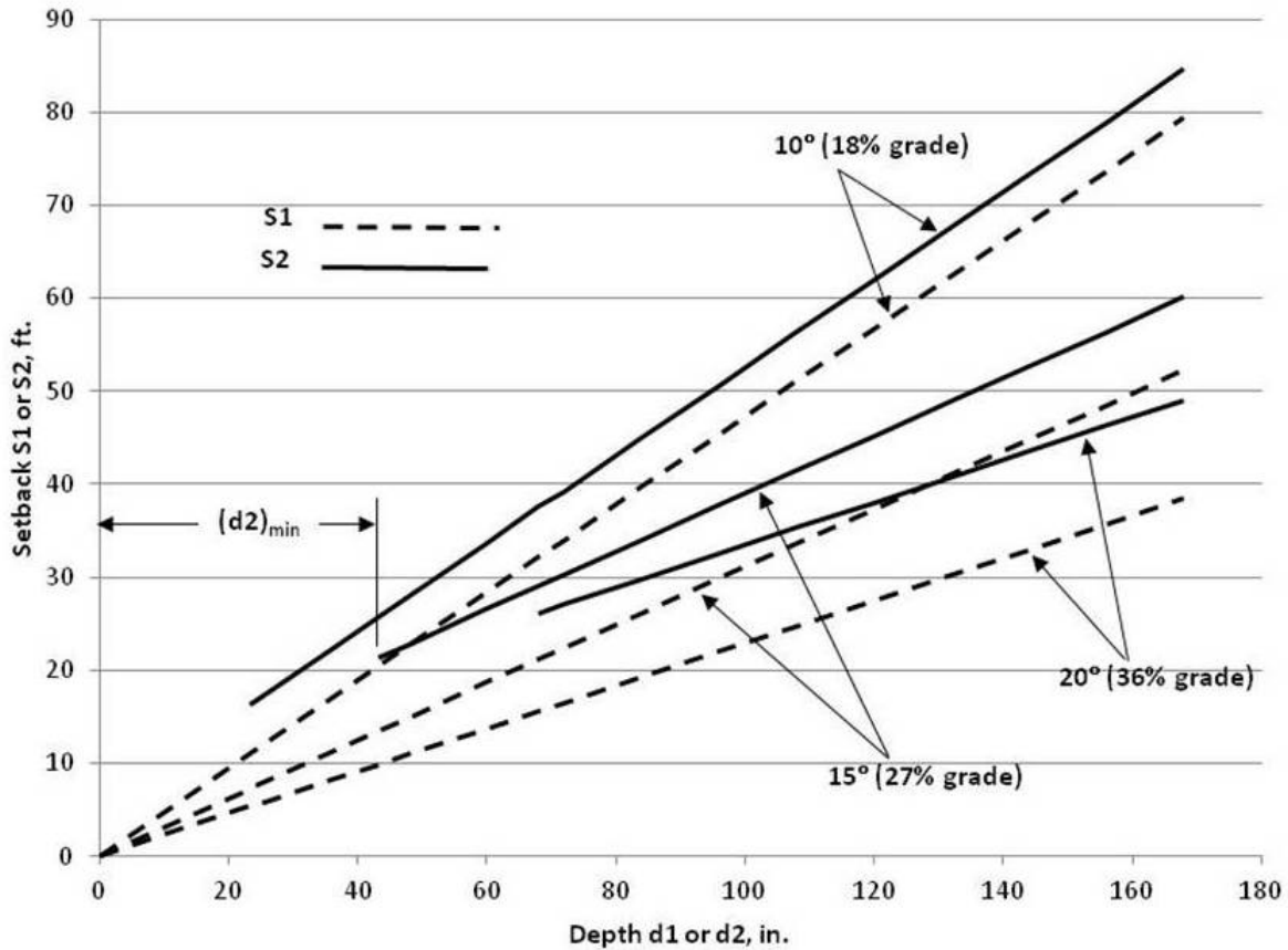
Figure 13 Drill Rig Setback Distance Drill Rods: 6 ft Long, 60 ft Radius of Curvature (Source: Outside Plant Consulting Services, Inc.)
