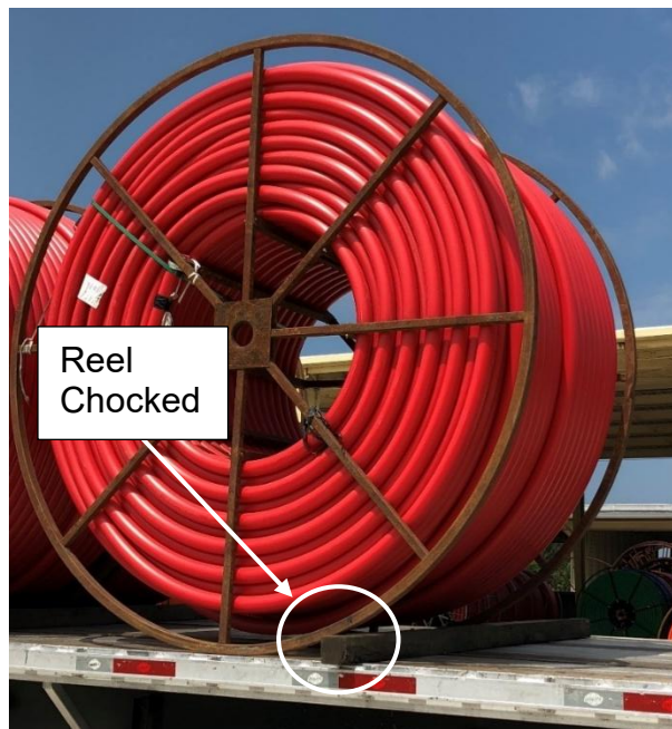
Figure 4 - PE conduit on a typical steel reel with blocking.
