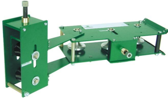
Figure 19 - Device for re-rounding and straightening HDPE conduit on reel or coils. This type of device is typically attached to a trailer with the pay-out reel.
