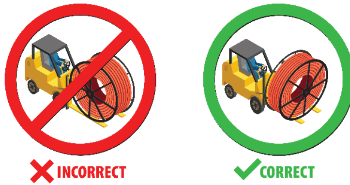
Figure 5 - Improper and proper handling of reels with a forklift. To prevent PE conduit damage, ensure that lifting forks are long enough to reach under, or through, both flanges of the reel so that all the weight of the reel is supported by the flanges and not by the conduit itself (Images available from PPI).
