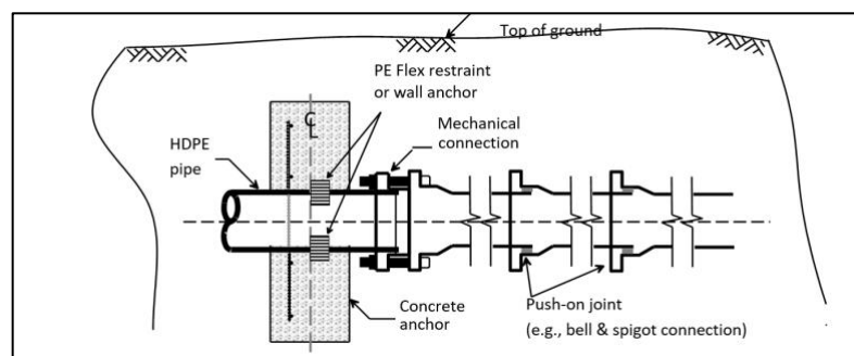
Figure A.2 Pullout prevention technique
