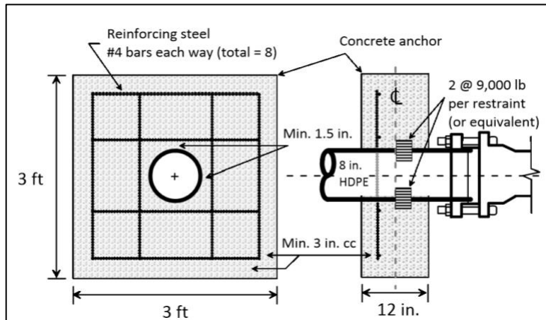
Figure A.3 Example: Reinforced Concrete anchor block for 8 in. HDPE DIPS DR13.5 pipe
