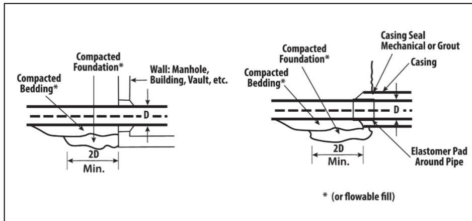
Figure 7 Controlling shear and bending
