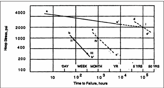
Figure 13 Hoop Stress vs Time to Failure
