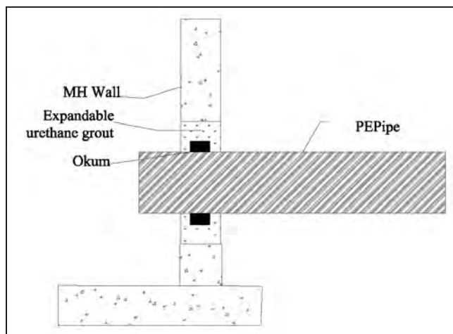
Figure 15 Connecting PE Pipe to Old Manhole
