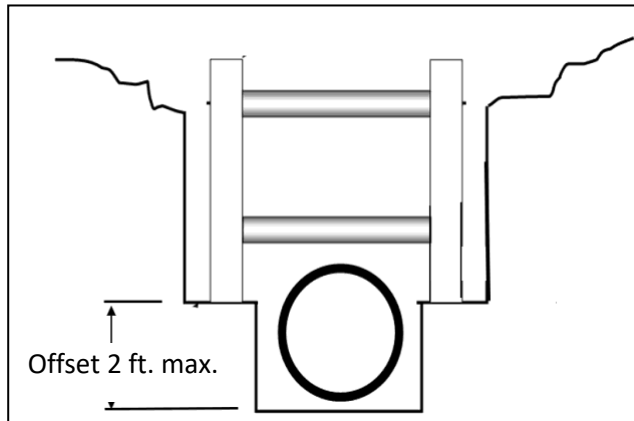
Figure 2 Trench Box Installation
