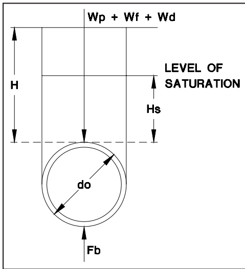
Figure 3-2 Prism Load
