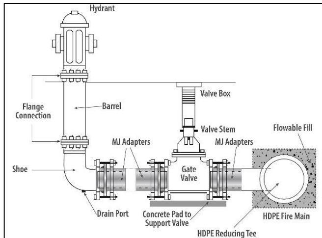
Figure 6 Typical Assembly and Support Arrangement for PE Pipe Connections to Valves and Hydrants
