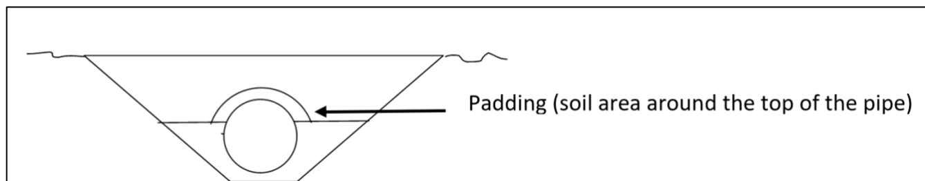
Figure 4 Soil Padding for Buried Pipeline in a trench with sloped walls
