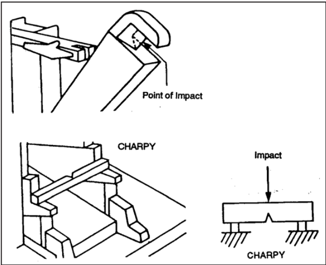
Figure 15 Charpy Test
