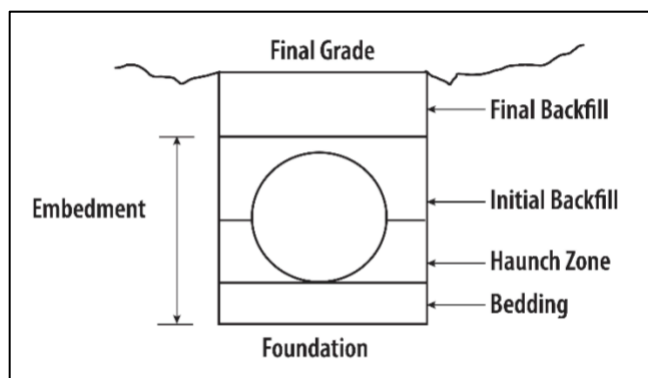
Figure 1 Trench Construction Terminology
