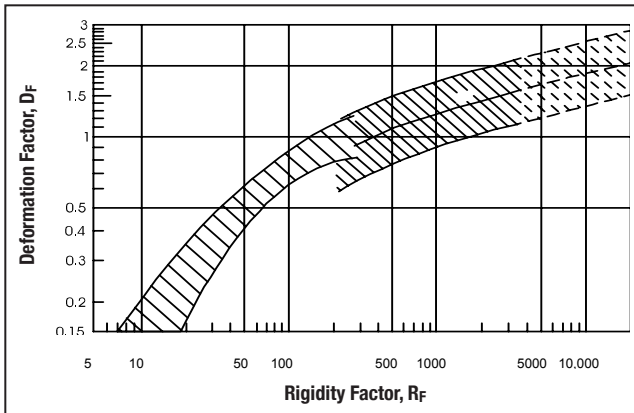
Figure 3-6 Watkins-Gaube Graph
