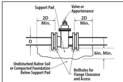
Figure 8 Appurtenance support (and consider use of valves with HDPE stubs)
