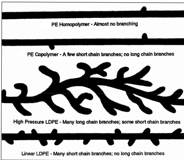
Figure 2 Chain Structure of PE
