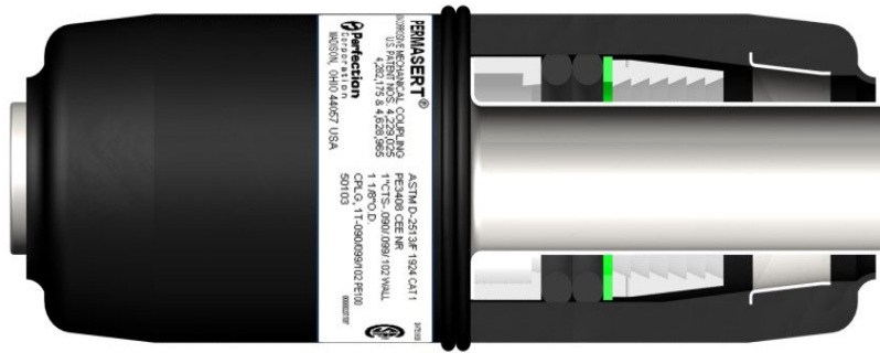
Figure 11 - Example of a stab fitting design showing stiffener, without pipe inserted (Courtesy of Perfection)
