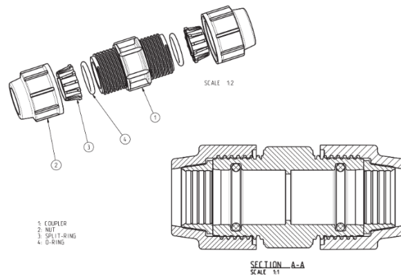
Figure 5 - Schematic of a compression nut fitting design (Courtesy of Plasson)
